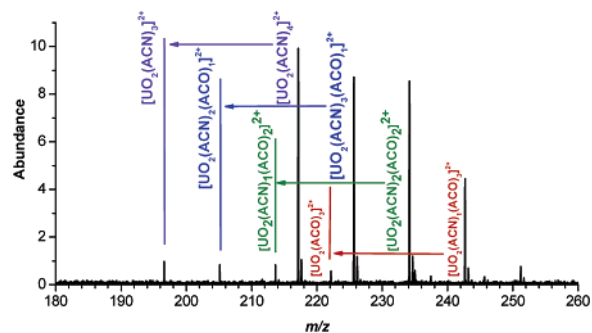
Figure 10. Mass spectra of mixed acetonitrile/acetone uranyl complexes [\text{UO}_2(\text{ACN})_m(\text{ACO})_n]^{2+} (where m + n = 4 ) isolated using SWIFT and photofragmented at 995 cm -1 . The experiment simultaneously produced IRMPD spectra for four different complexes.
