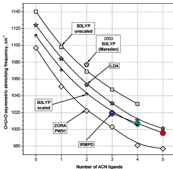
Figure 9. Comparison of O=U=O asymmetric stretching frequencies for the [\text{UO}_2(\text{ACN})_n]^{2+} complexes measured using IRMPD and calculated using B3LYP (scaled and unscaled), LDA, and ZORA-PW91 levels of theory.
