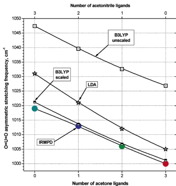
Figure 12. Comparison of O=U=O asymmetric stretching frequencies for the [UO_2(ACN)_m(ACO)_n]^{2+} complexes ( m+n=3 ) measured using IRMPD and calculated using B3LYP and LDA levels of theory.
