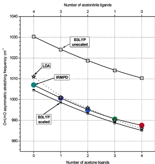
Figure 11. Comparison of O=U=O asymmetric stretching frequencies for the [UO_2(ACN)_m(ACO)_n]^{2+} complexes ( m+n=4 ) measured using IRMPD and calculated using B3LYP and LDA levels of theory.
